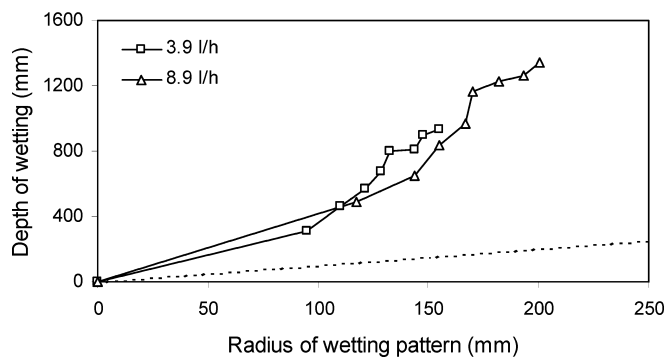
Fig. 4 The radius of a wetting pattern from drip irrigation plotted against the estimated depth of the wetting pattern for fast and slow emitters on a loamy sand soil. The dotted line represents a hemispherical wetting pattern where the depth is equal to the radius at the surface
