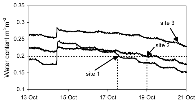
Fig. 2 The water content measured by TDR during a drying cycle and the day to irrigate based on a refill point of 0.2 \text{ m}^3 \text{ m}^{-3}
