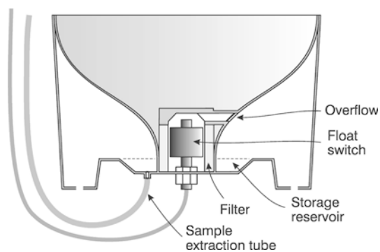
Fig. 5 A schematic of the wetting front detector showing the filter, cavity, float switch and overflow reservoir for collection of soil solution
