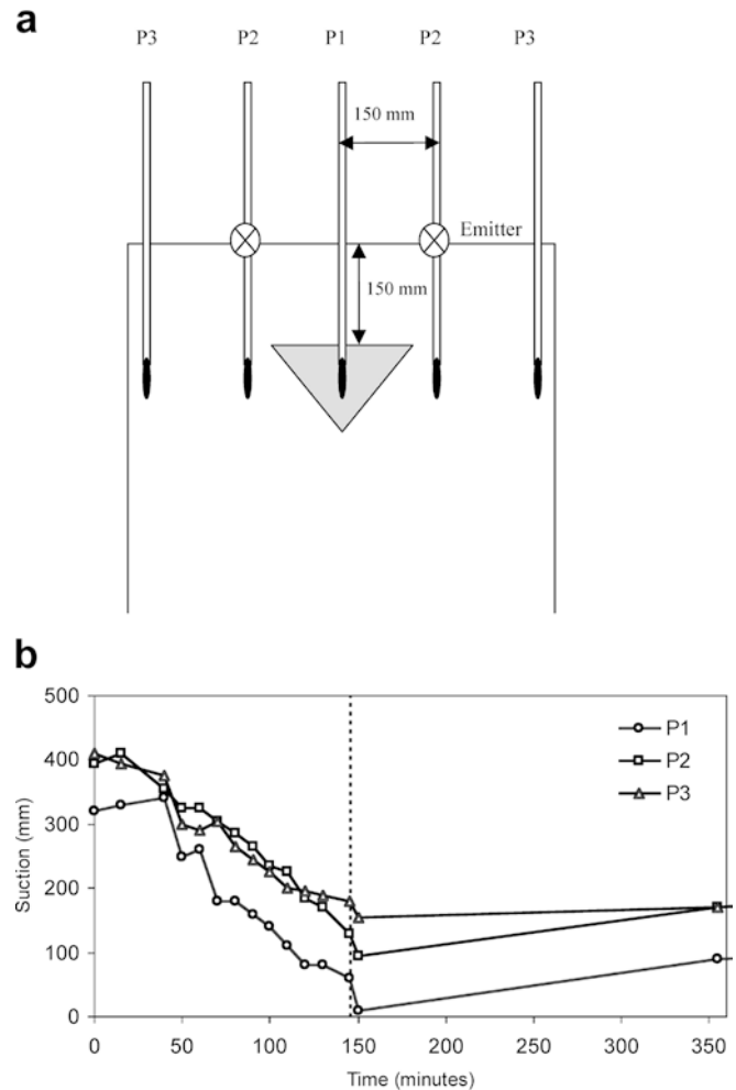
Fig. 6 a The location of tensiometers around a buried detector. Position 1 ( P1 ) was inside the detector, position 2 ( P2 ) directly beneath an emitter and position 3 ( P3 ) 150 mm away from the emitter. b The change in soil suction during irrigation inside and outside the detector. The vertical dotted line shows the time the float detected water and the irrigation system was turned off
