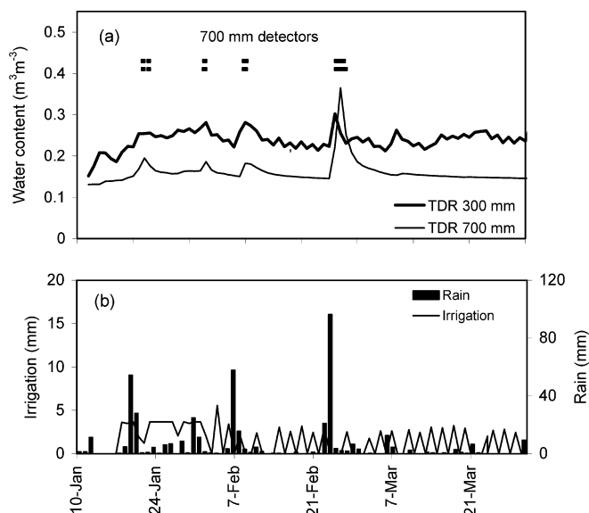
Fig. 7 a The continuous lines show the average water content (TDR) at 300 and 700 mm depths from a drip-irrigated capsicum crop. The horizontal broken lines at the top of the figure show the times when the deep detectors (two replicates) recorded water ( start of the line ) and the time the water was withdrawn from the funnel by capillary action ( end of the line ). b the amount of irrigation and rain received during the growing season
