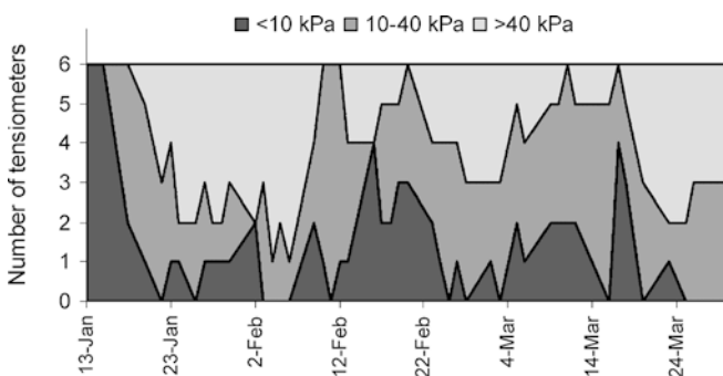
Fig. 1 The number of tensiometers reading a suction of < 10 kPa, 10–40 kPa, > 40 kPa in a melon crop before irrigation. All six tensiometers were in the 10–40 kPa zone on just one day (11 February)
