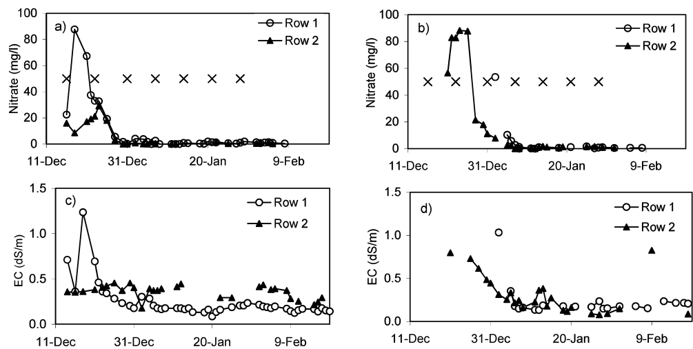
Fig. 9 a The nitrate concentration measured at 200 mm. X marks the time of fertigations. b The nitrate concentration measured at 500 mm. c The electrical conductivity (EC) measured at 200 mm. d The EC measured at 500 mm
